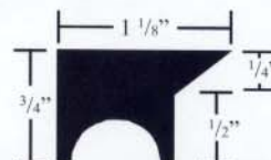
R214 RUBBER 275-300- Temp. Deg. F
